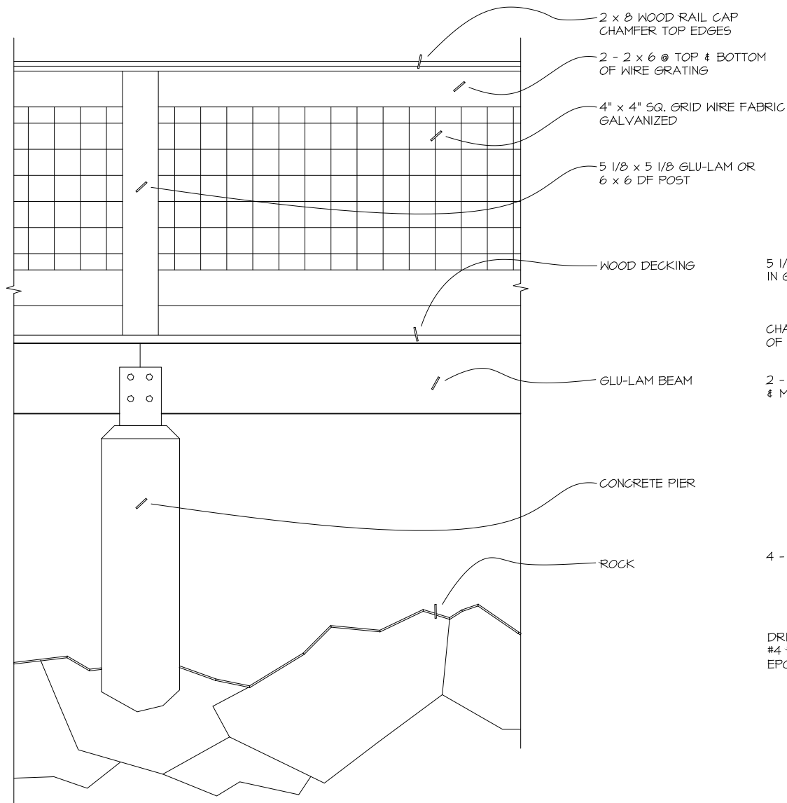
WALKWAY ELEVATION NO SCALE
