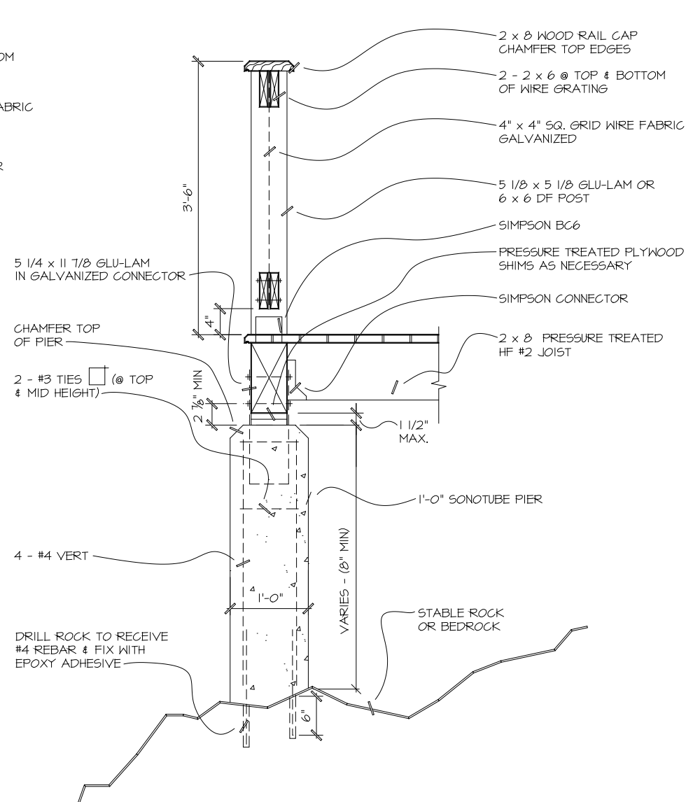
1 WALKWAY PIER ON ROCK NO SCALE
